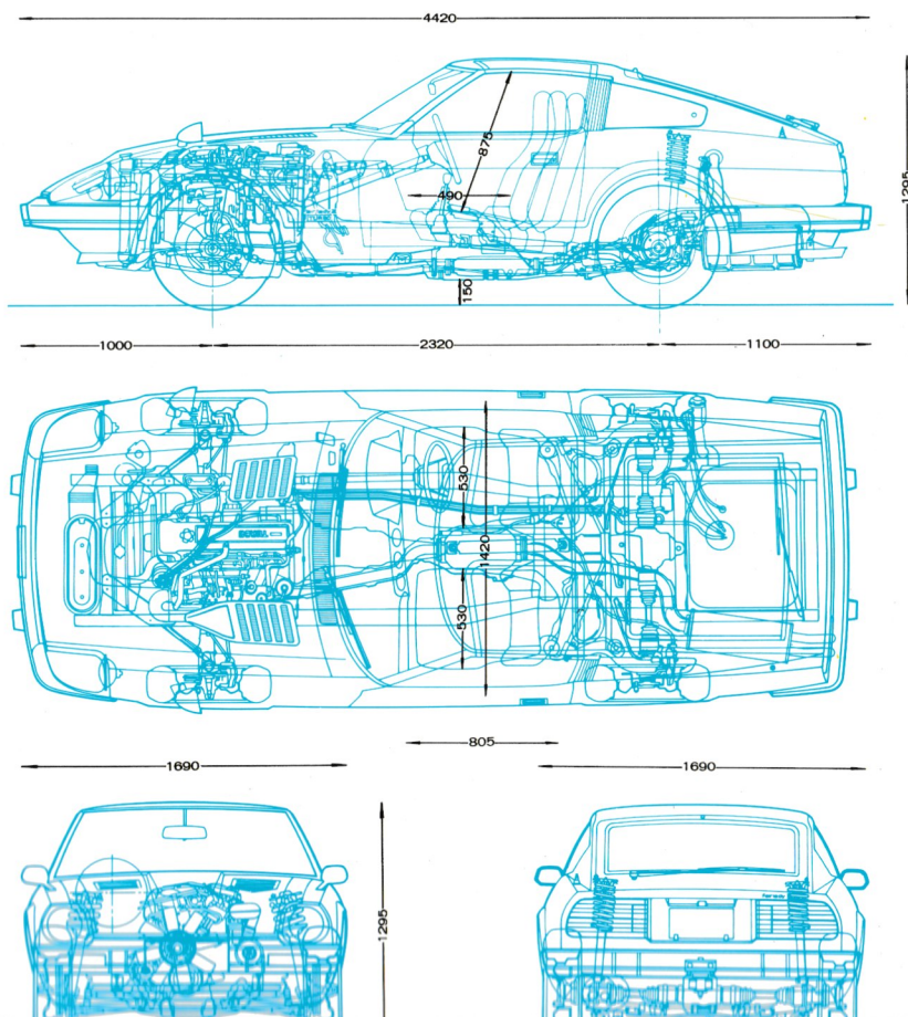
2SEATER(T-BAR ROOF TURBO)
