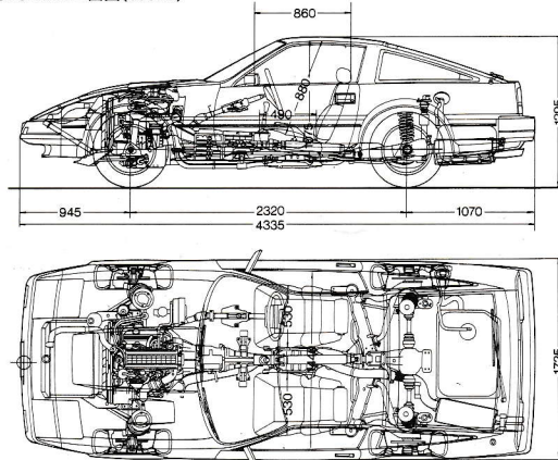
●2SEATER二面図(300ZX)
