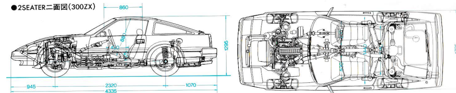
●2SEATER二面図(300ZX)
